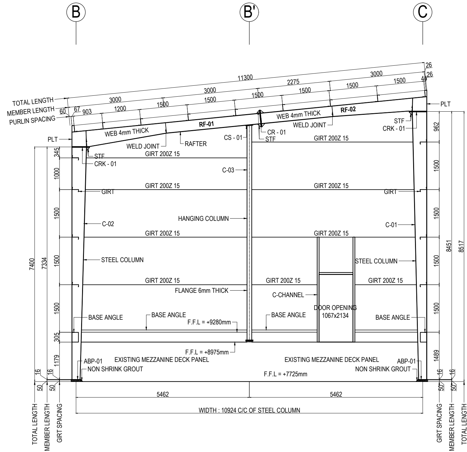
END WALL FRAMING @ GRID - 6
